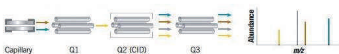
Figure 6. Schematic diagram of triple quadrupole mass analyzer.
